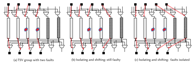
FIGURE 1. Illustration of shifting method with two spare TSVs. The parity check is used to detect and localize the fault. Red dotted arrow is the configuration to isolate and localize the fault.
