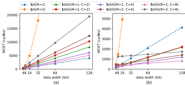
FIGURE 4. Comparison of worst case execution time (WCET) between IaS and IaSiG with K = 32 : (a) case-1; (b) case-2.
