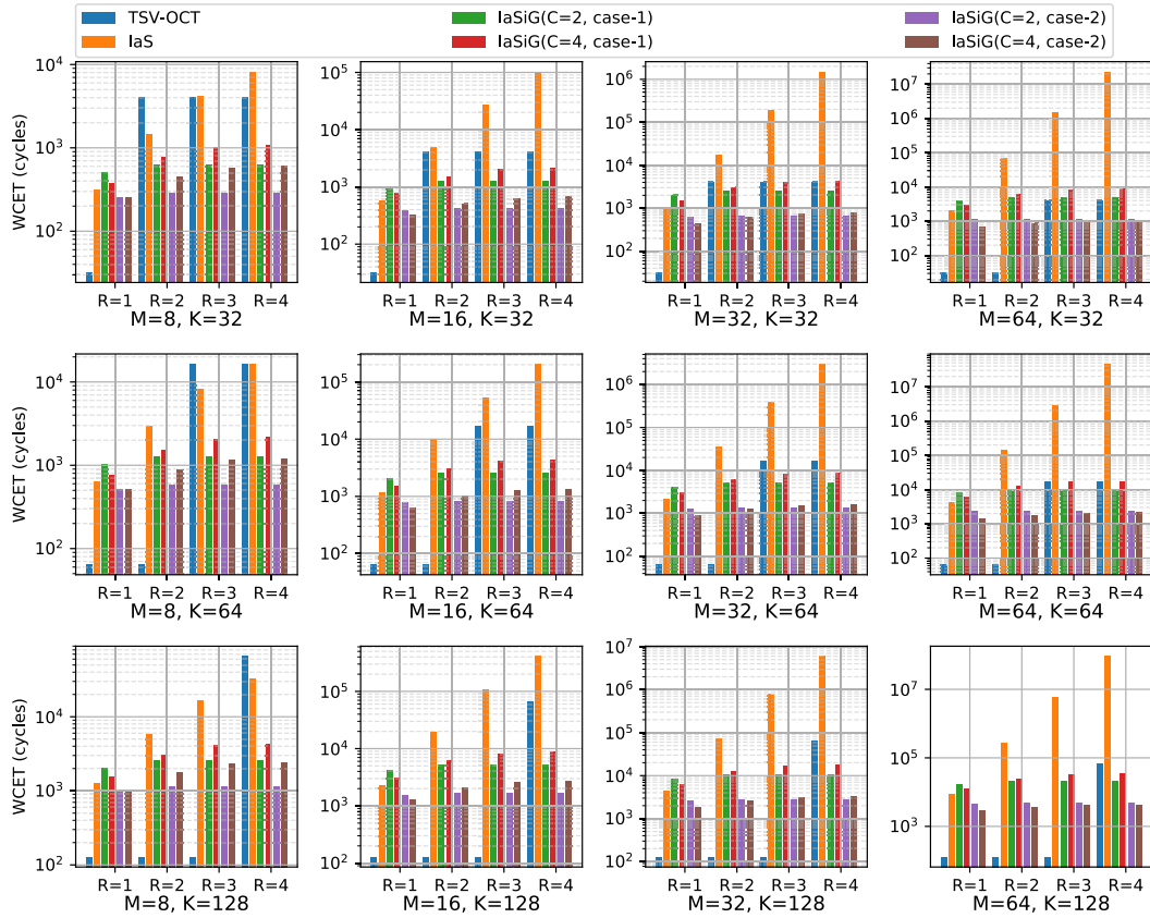
FIGURE 8. Comparison of worst case execution time (WCET). Note that the WCET of IaSiG are in case-1 and case-2 (see Section III-B). With TSV-OCT [35], R is the number of defective TSVs.
