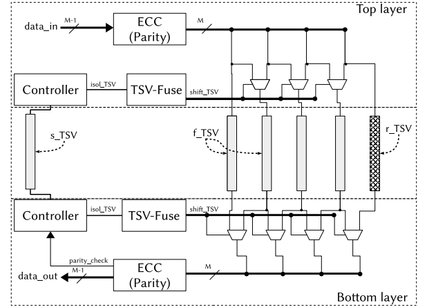
FIGURE 2. IaS architecture for M = 4 , R = 1 [27]. s\_TSV : synchronization TSV; f\_TSV : functional TSV; r\_TSV : redundant TSV.
